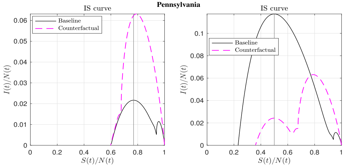
Figure 25: The IS curves under the two forecast scenarios with an initial delay of 5 days.
